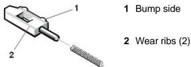
Figure 21. Left Bay Latch and Spring
