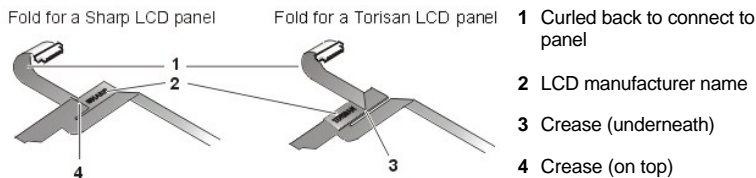
Figure 16. 12.1-Inch LCD Flex Cable
