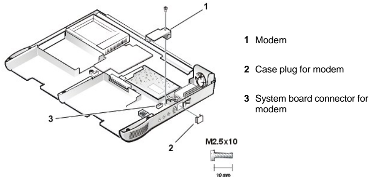
Figure 22. Modem Assembly
