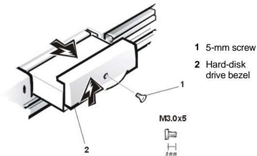
Figure 6. Hard-Disk Drive Assembly
