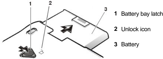
Figure 2. Main Battery Assembly Removal
