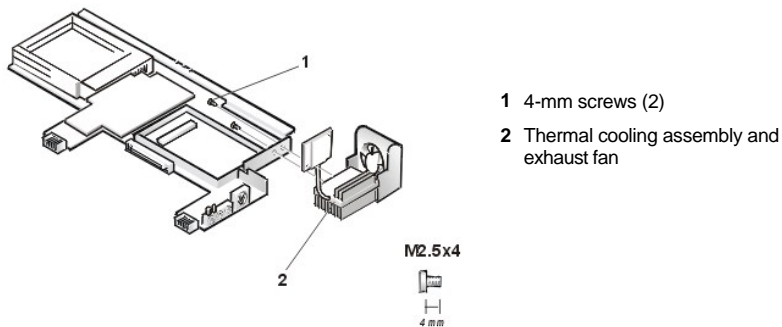
Figure 24. Thermal Cooling Assembly
