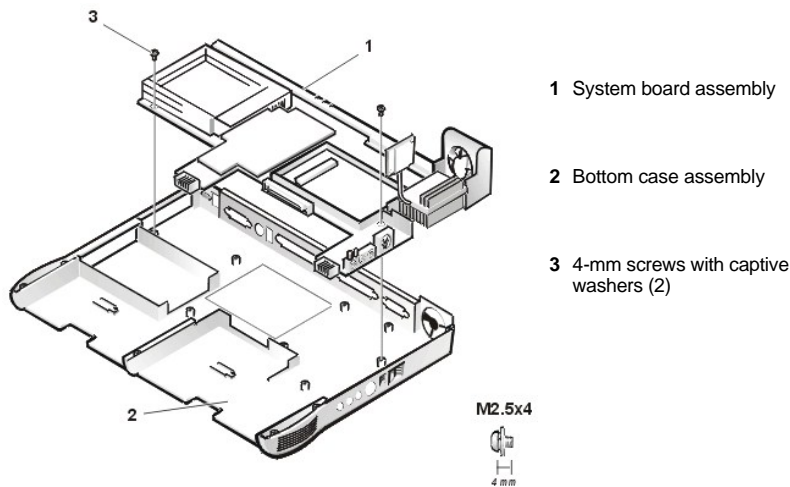
Figure 23. System Board Assembly
