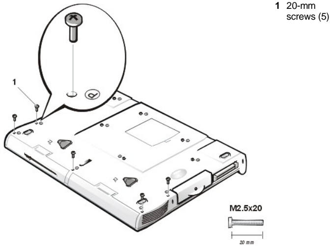
Figure 18. Removing the Palmrest Assembly Screws
