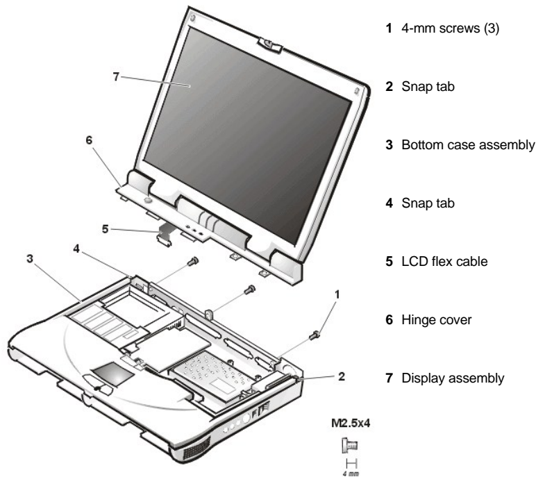
Figure 13. Display Assembly
