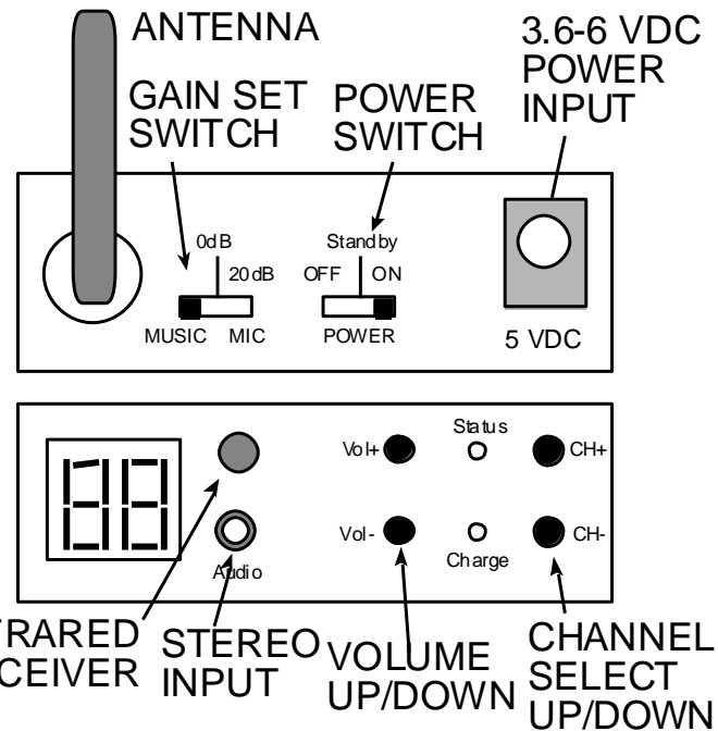
Fig 2: WLT-02 TRANSMITTER
