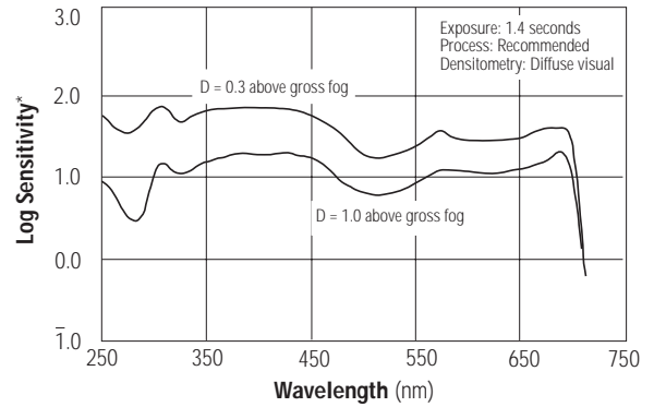
Spectral Sensitivity
