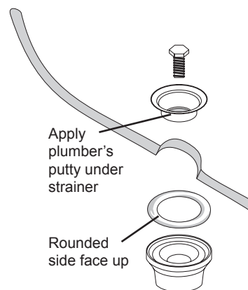
FIGURE 7. Strainer assembly
