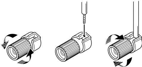
Loosen the Terminal Insert the core Tighten the Terminal Connection of speaker cable Terminal
