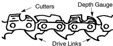
Drive Links
