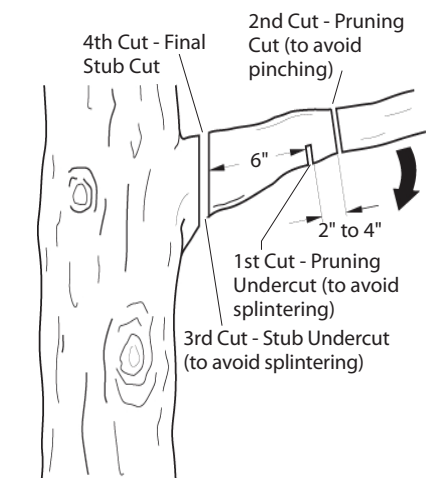
Figure 20 - Cutting A Limb
