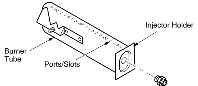
Figure 23 - Injector Holder On Burner Tube
