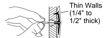
Figure 5 - Popping Open Anchor Wings For Thin Walls
