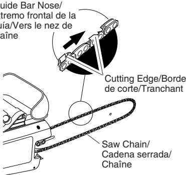
Figure 2 - Chain Position
