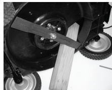
Figure 26 - Wedging the Wood
