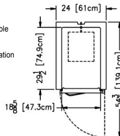
Plan - R/ALT132DUT
