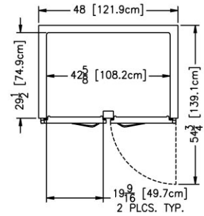
Plan - R/ALT232DUT
