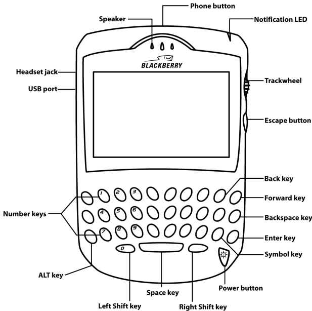
The BlackBerry 6200 Series of Wireless Handhelds
