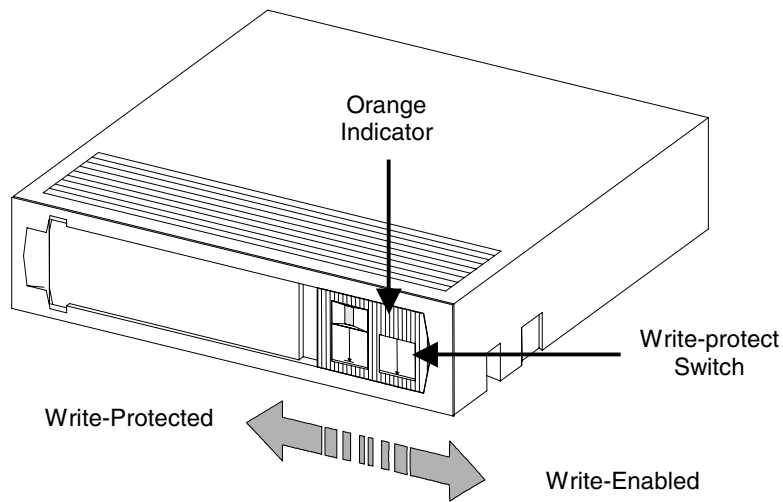
Figure 5. DLT Data Cartridge
