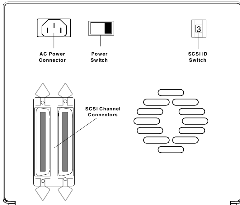
Figure 4. DS9000 Series Rear Panel
