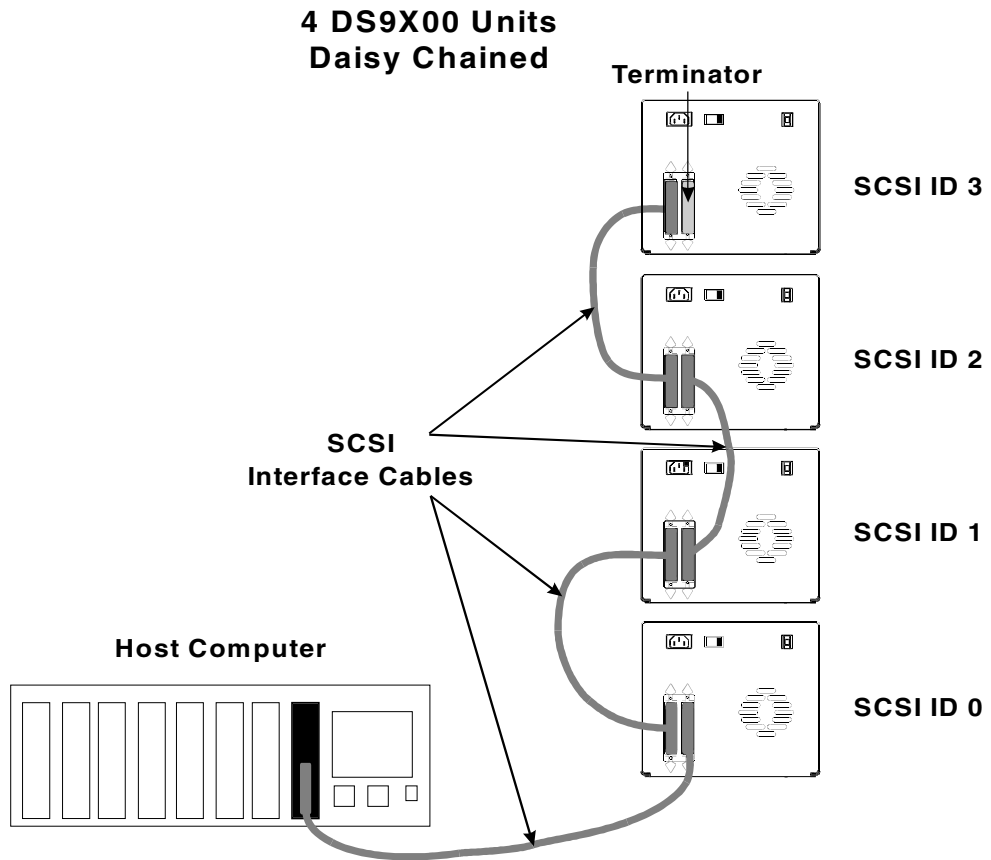
Figure 6. Cable Diagram for 4 DS9000 Series Units
