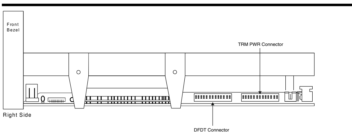
Figure 15. DLT7000/DLT8000 Tape Drive Connectors (right side)
