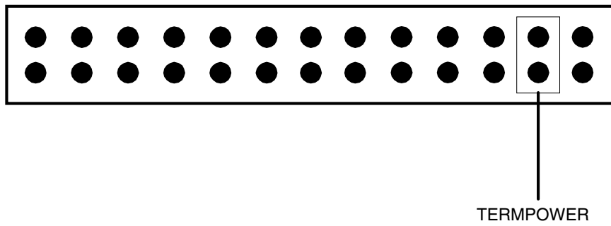
Figure 16. Term Power Pins on TRM PWR Connector
