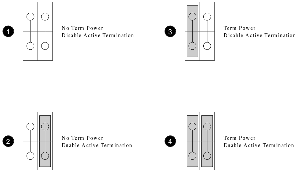
Figure 14. TRM PWR/TRM ENB Jumper Positions
