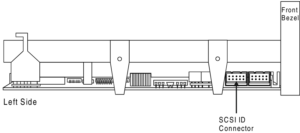
Figure 9. DLT4000 Tape Drive Connectors (left side)
