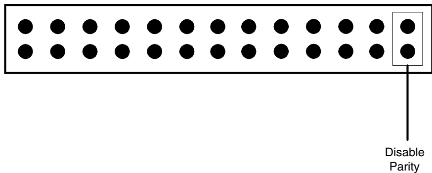
Figure 12. Disable Parity Pins on DFDT Connector
