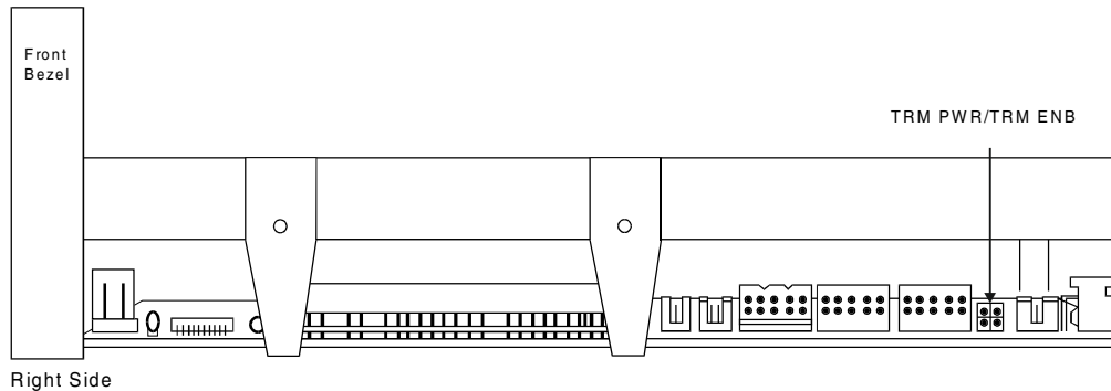
Figure 13. DLT4000 Tape Drive Connectors (right side)
