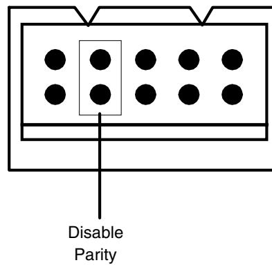
Figure 10. Disable Parity Pins on SCSI ID Connector
