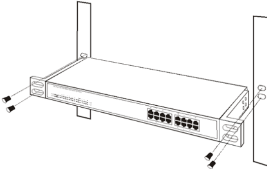
Figure 2. Attach Switch to Rack
