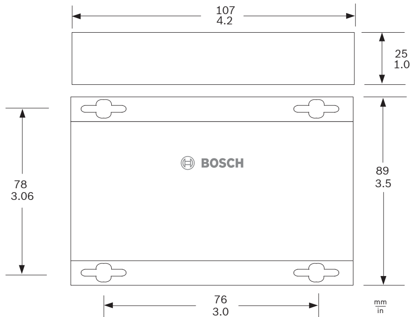
Figure 13 Stand-alone Modules: LTC 4642/50, LTC 4642/60, LTC 4651/60, LTC 4651/50
