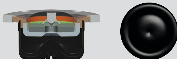
Shown above, the EWB tweeter's unique design features a diaphragm that is terminated at its center.
