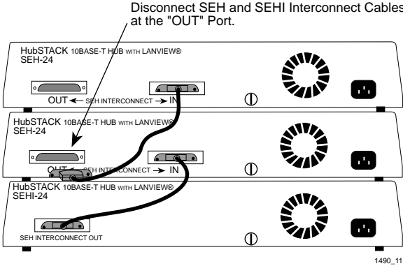
Figure 3-7. Disconnecting the HubSTACK Interconnect Cable
