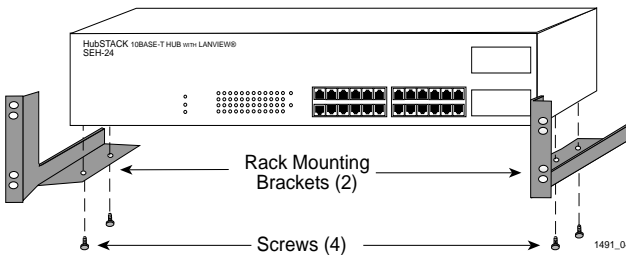
Figure 3-4. Installing the Rack Mount Brackets
