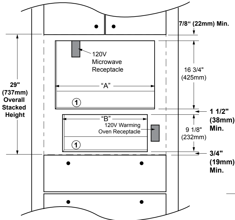
CUTOUT DIMENSIONS DMT2420 SHOWN
