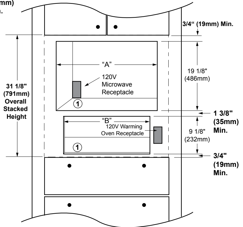
CUTOUT DIMENSIONS DCM24 SHOWN
