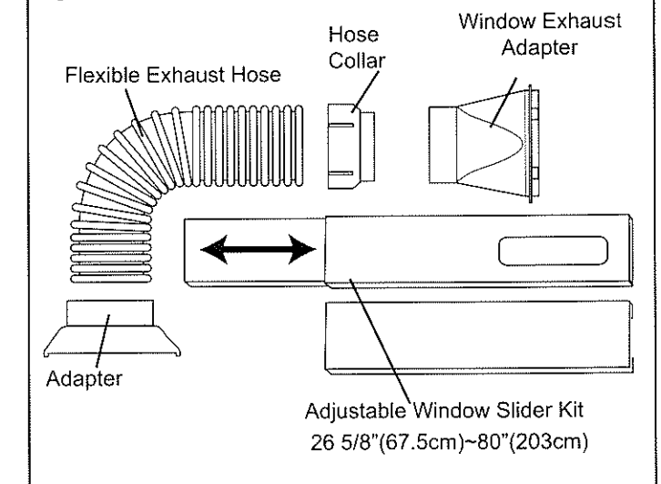
Fig. 1 Installation Accessories
