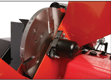
Heavy duty rotor disc that features two reversible heat treated steel chipper blades
