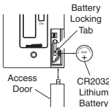
Removing Access Door and Battery
