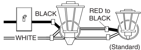
Wiring to Motion Light & Standard Fixture
