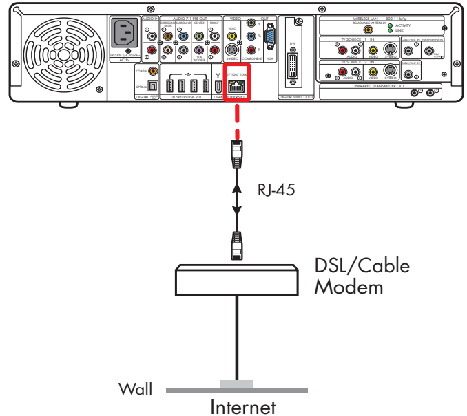
DSL/Cable modem direct Internet connection
