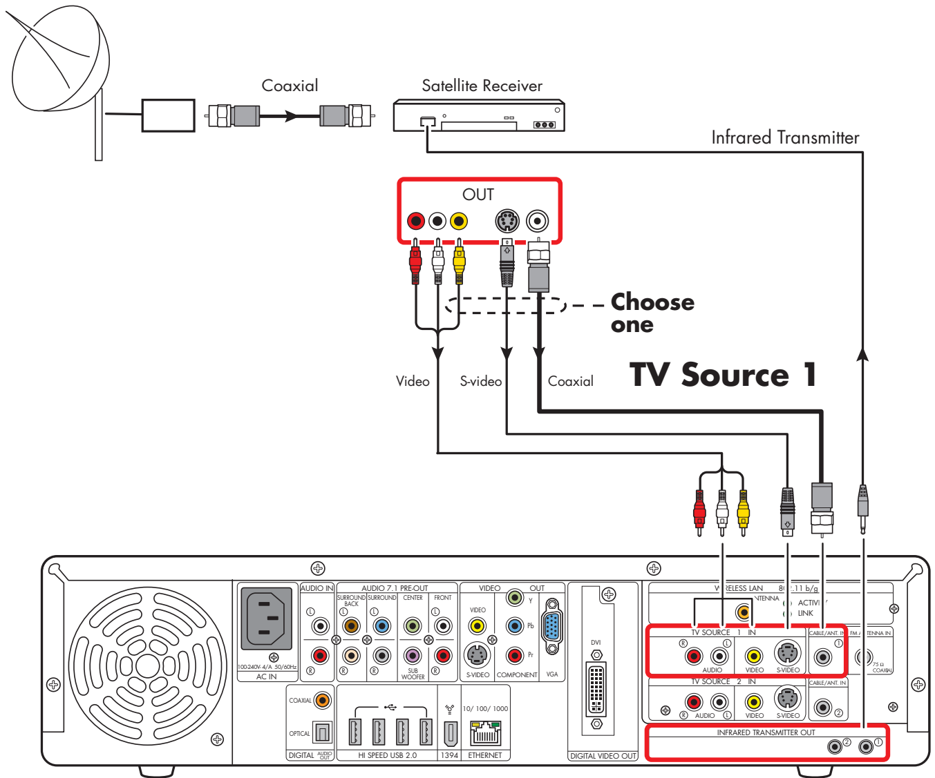
TV signal source – one satellite receiver
